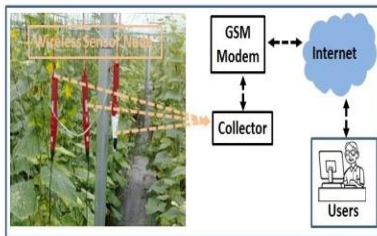
Fig.1 WSN Architecture
