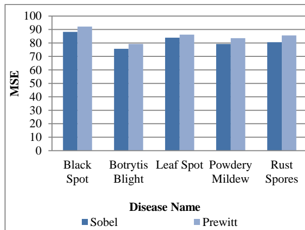
Figure 17. MSE Comparison
