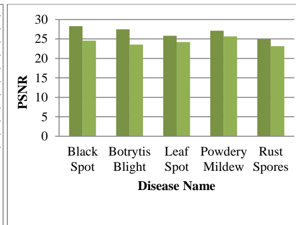
Figure 18. PSNR Comparison
