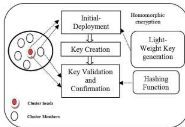
Fig. 2: TKMP Architecture
