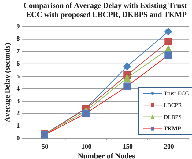
Fig. 15. Chart of packet delay ratio.
